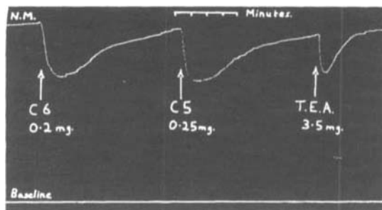
FIG. 10.—Cat, chloralose. Record of sustained contraction of nictitating membrane excited by stimulation of cervical sympathetic 10 sec. intravenous injections. Effects of 0.2 mg. C6; 0.25 mg. C5; and 3.5 mg. tetraethylammonium iodide (T.E.A.).
